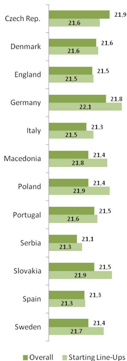
Average Age
